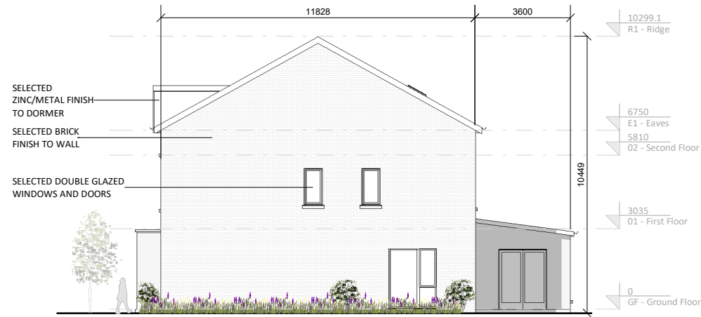
① H06A Side Elevation (End of Terrace) 1 : 200
